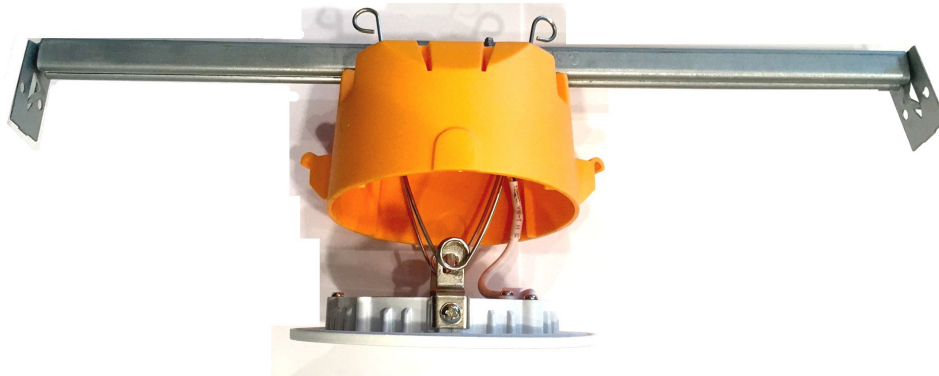
AL-CBOX4 mounting hanger bar
