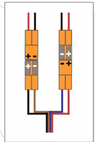
Connection Detail
