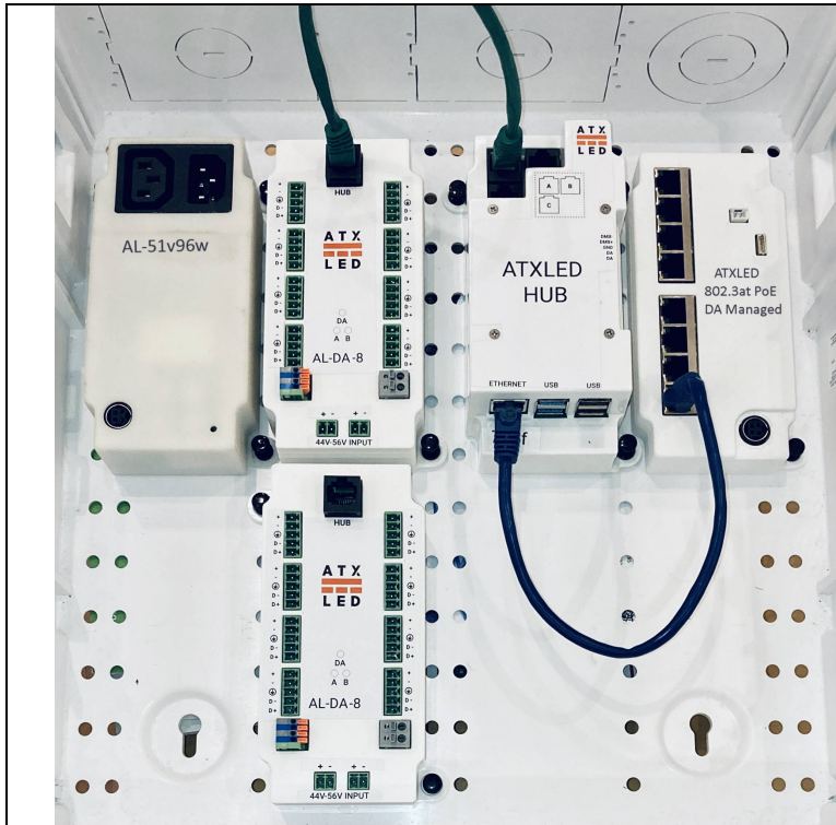
Structured Wiring DALI power supply with easy wiring
