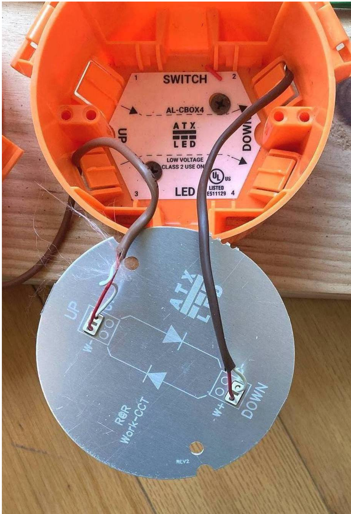
Close up of the Work light wiring
